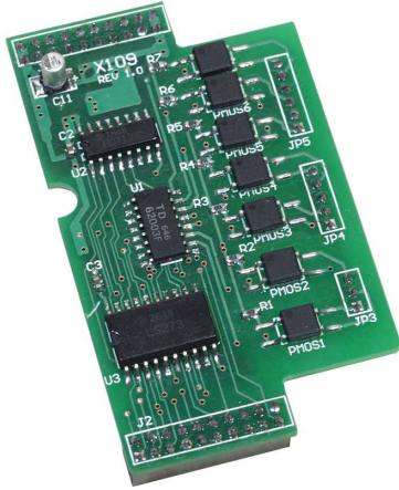
X109 7-channel PhotoMos relay
